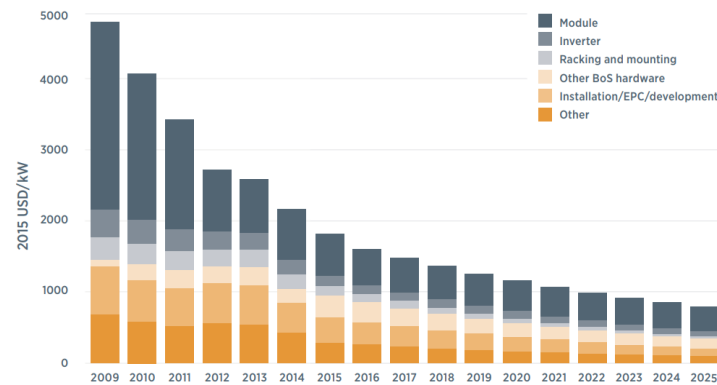
Figure 1. System cost breakdown for utility-scale photovoltaics: Global weighted average (Source: IRENA, 2017)
